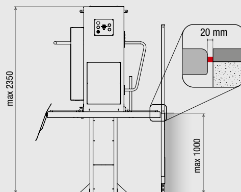
FRONT VIEW: overall height at max extension
